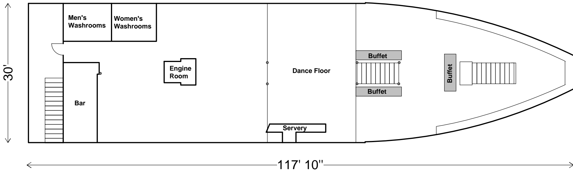
NORTHERN SPIRIT LOWER DECK
